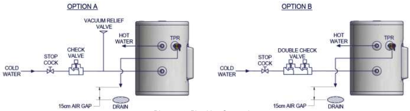
Diagram 3. Plumbing Connection
